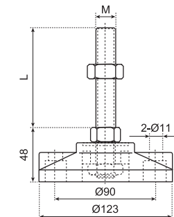
FD123 塑料底盘固定底脚 FD123 PLASTIC BASE FIXED FEET
