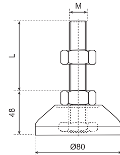
FD80 塑料底盘固定底脚 FD80 PLASTIC BASE FIXED FEET
