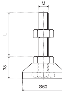
FD60 塑料底盘固定底脚 FD60 PLASTIC BASE FIXED FEET
