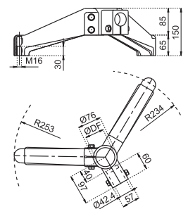
N108 120° 方型两爪半脚架 N108 SUPPORT BASE (BIPOD 120° WITH JOINT)
