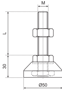
FD50 塑料底盘固定底脚 FD50 PLASTIC BASE FIXED FEET
