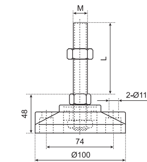
FD100 塑料底盘固定底脚 FD100 PLASTIC BASE FIXED FEET
